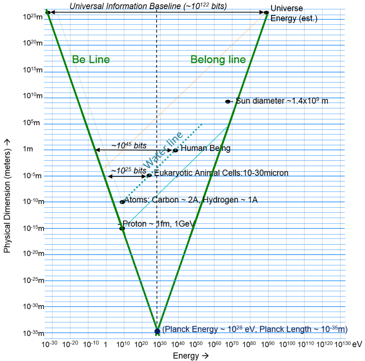
Figure 3: Information limits
