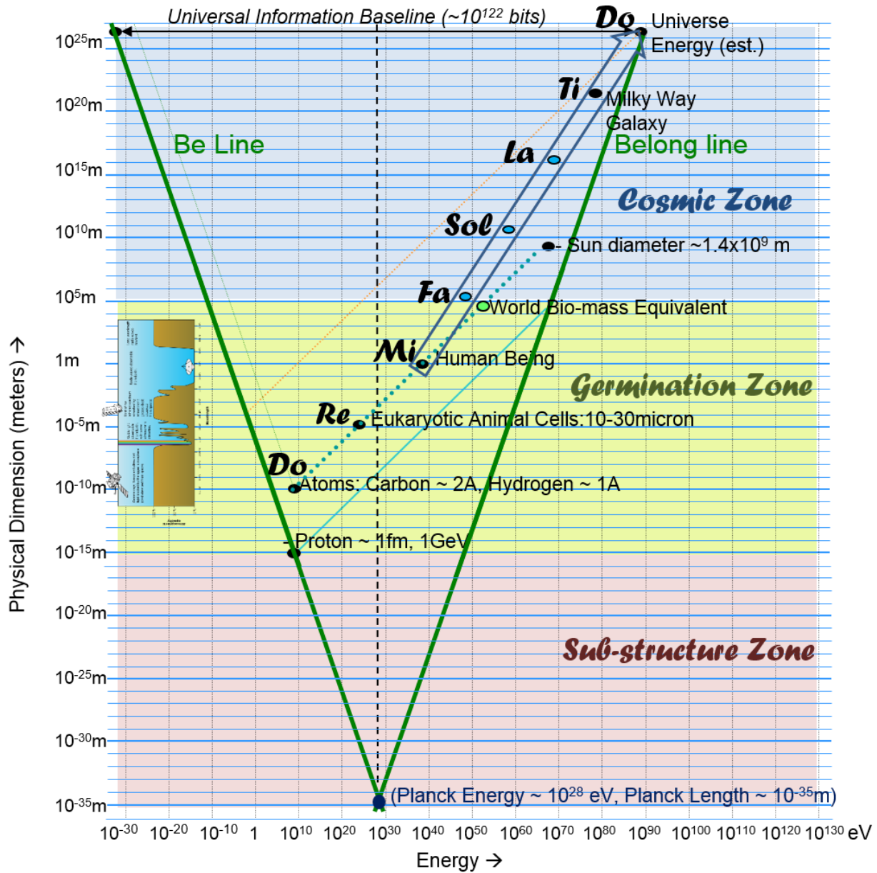
Figure 6: Cosmic Escalator
